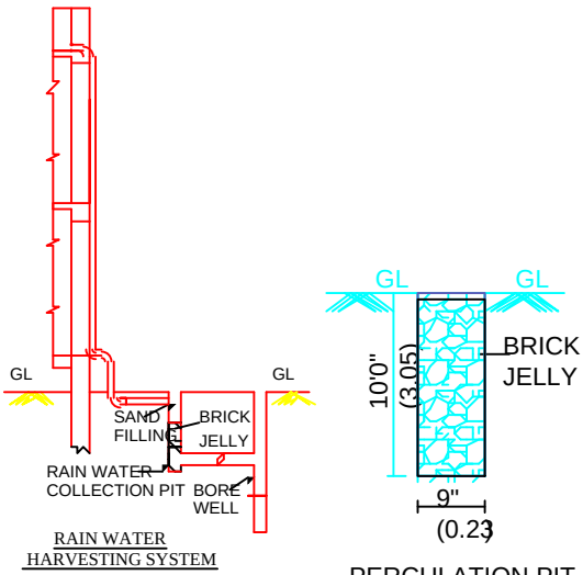
PERCOLATION PIT
