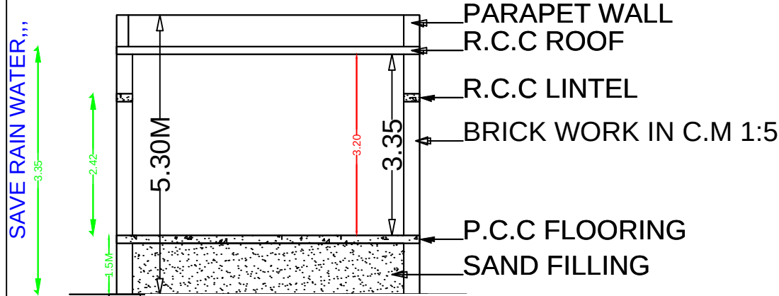
FOUNDATION
