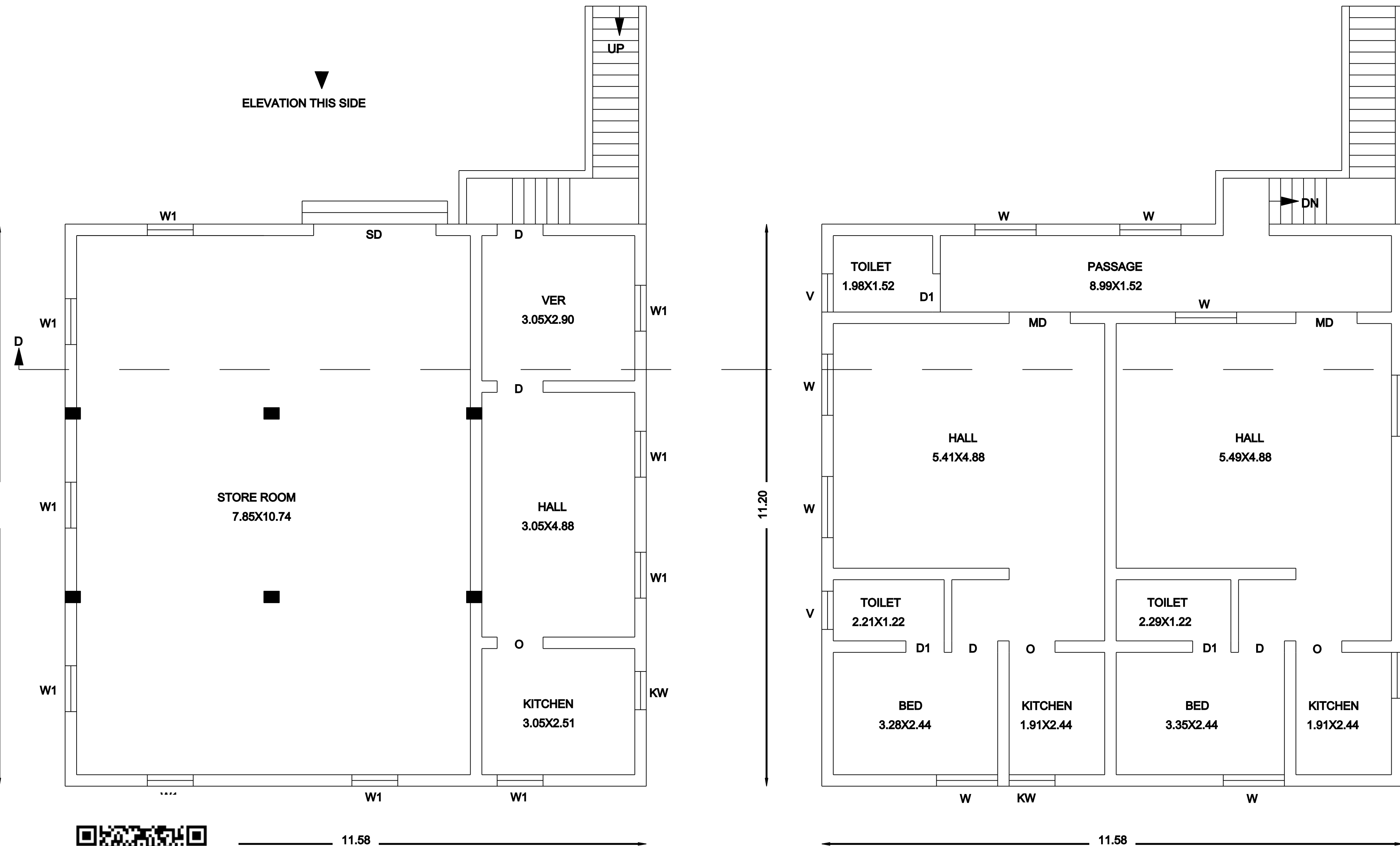
1 ST FLOOR PLAN (EXISTING)
