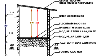
(BLK-1) SECTION AA
