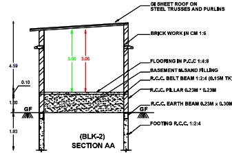
(BLK-2) SECTION AA
