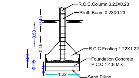
DETAILS OF COLUMN FOOTING
