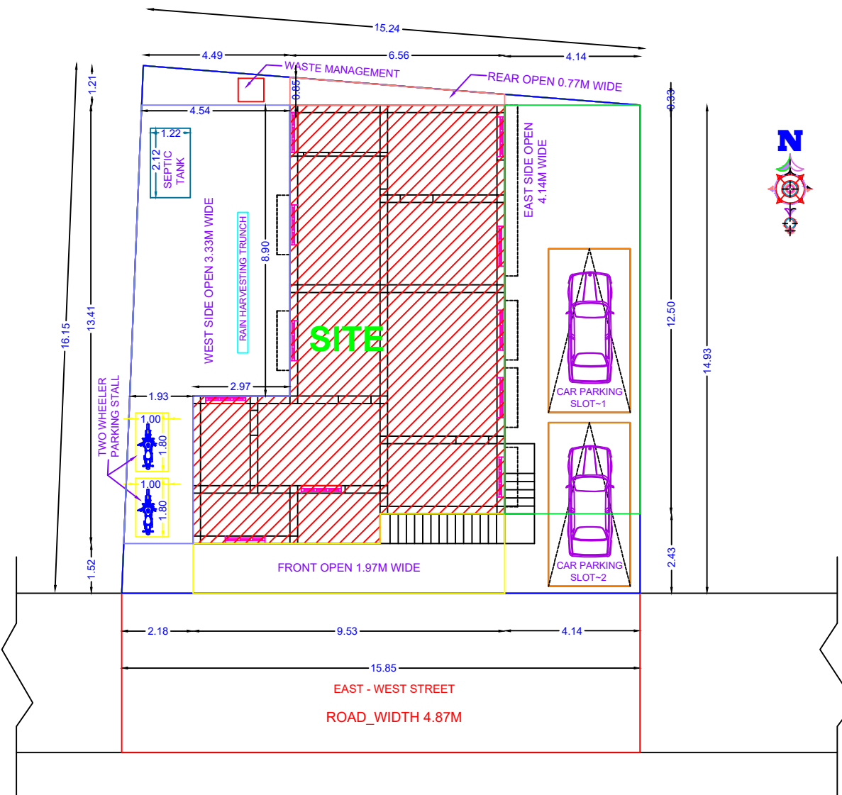
SITE PLAN
