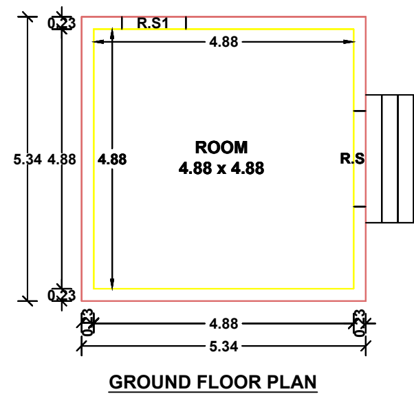
DETAIL PLAN SCALE :- 1:100
