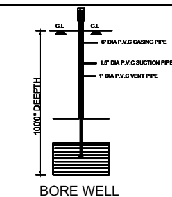
BORE WELL
