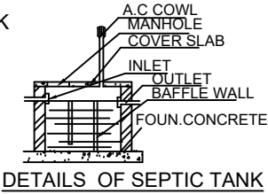
DETAILS OF SEPTIC TANK
