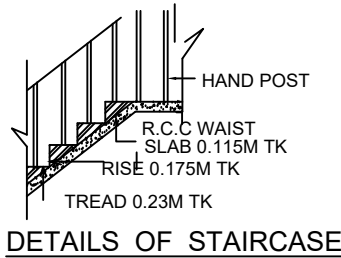
DETAILS OF STAIRCASE
