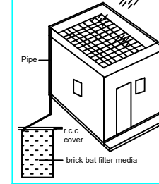
RAIN WATER STORAGE
