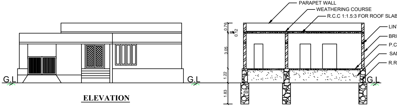
SECTION ON "DC"
