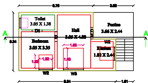
PRO GROUND FLOOR PLAN
