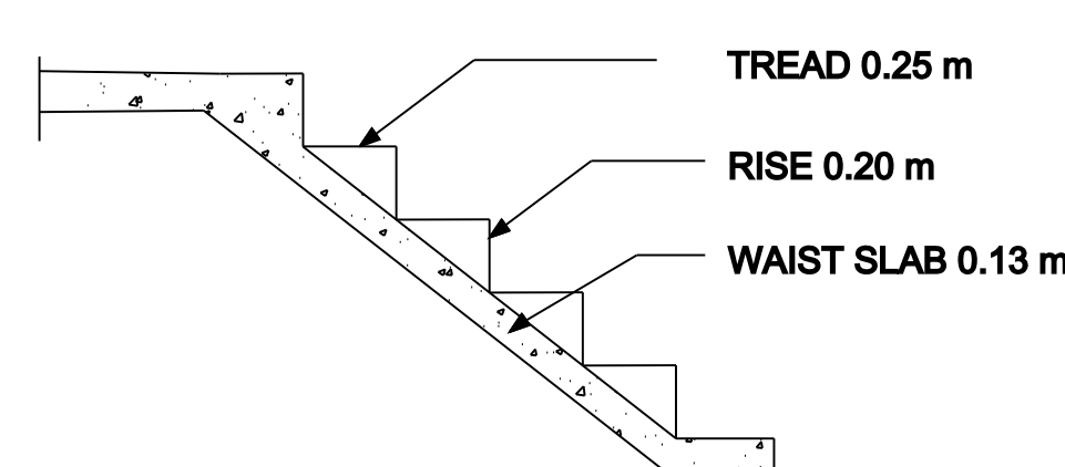
STAIR DETAILS
