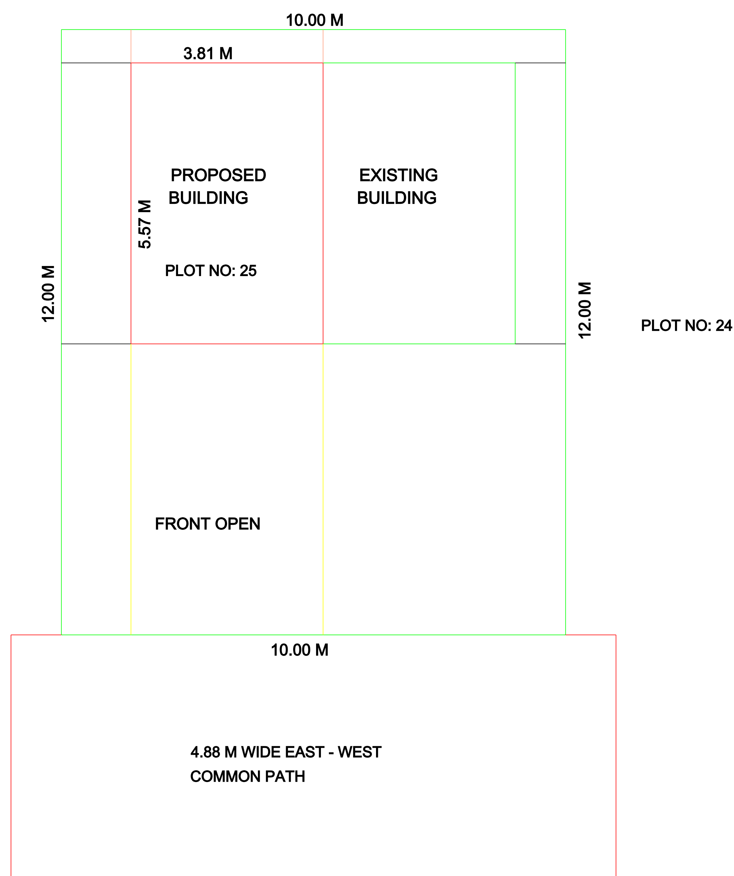
SITE PLAN
