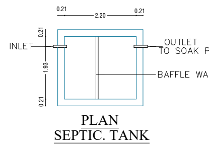
PLAN SEPTIC TANK
