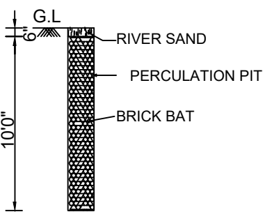
PERCULATION PIT
