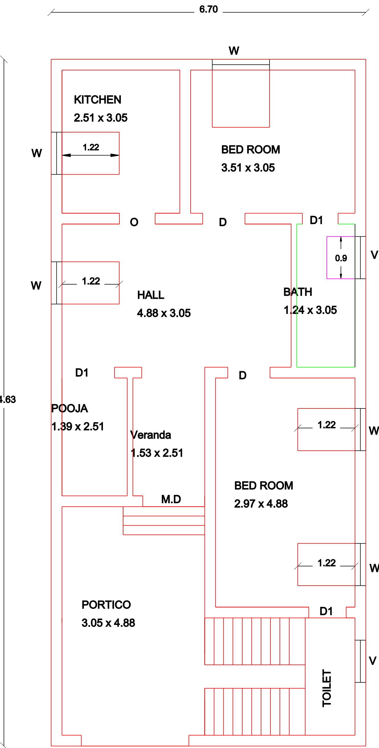
PLAN
