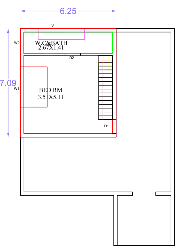
PRO PRO FIRST FLOOR
