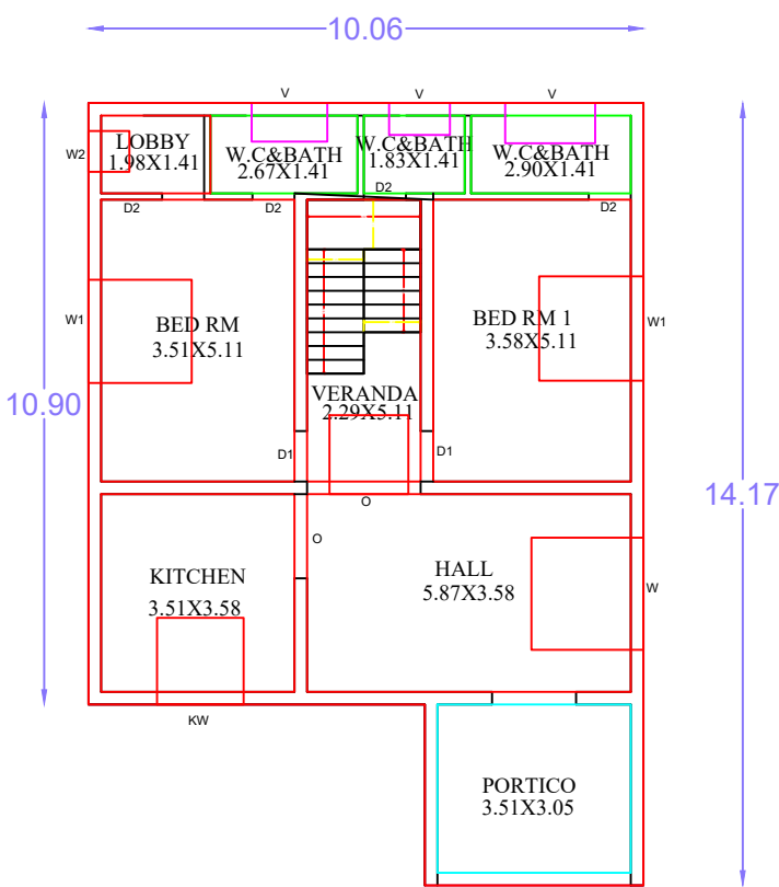
EX GROUND FLOOR
