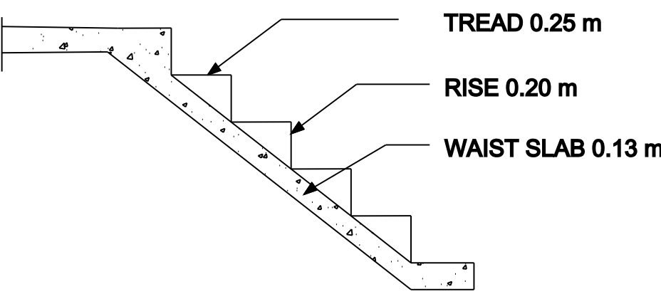
STAIR DETAILS
