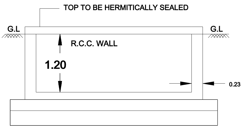
RWH_CAPACITY_L = 2000
