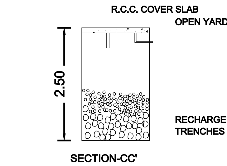
SECTION-CC'
