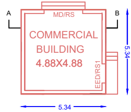
BUILDING PLAN SCALE 1:100
