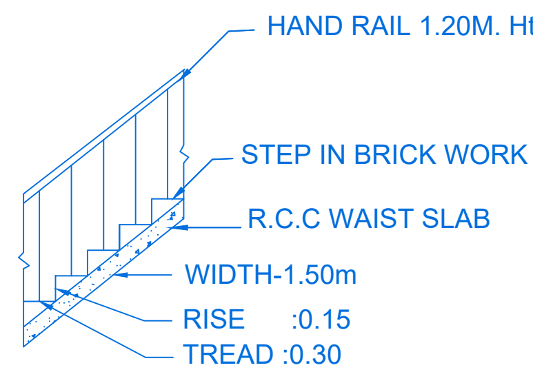
STAIR DETAIL
