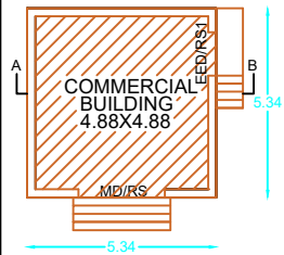
BUILDING PLAN SCALE 1:100
