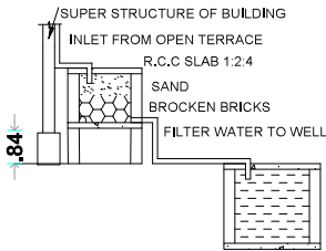
RAINWATER HARVESTING
