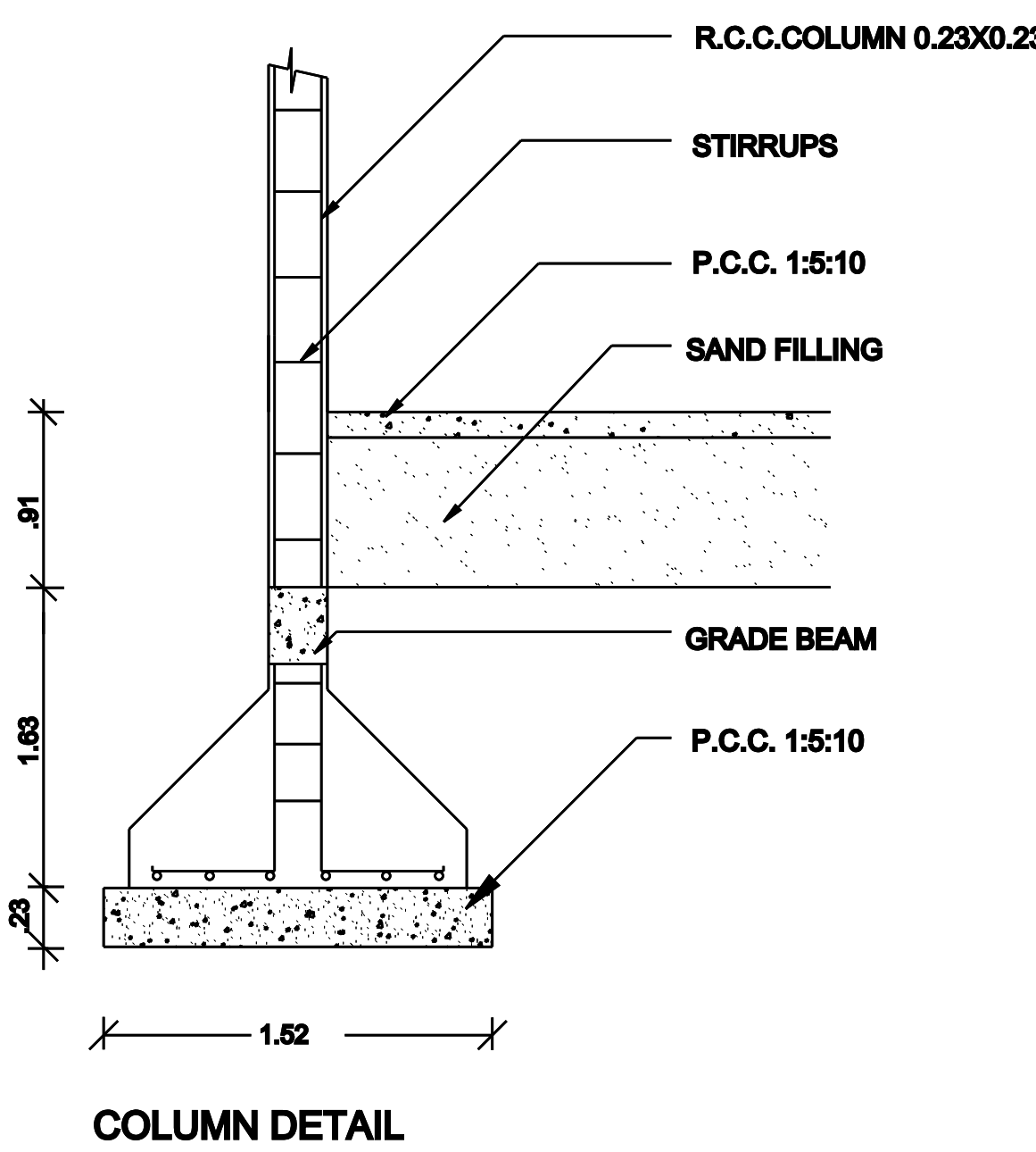
COLUMN DETAIL
