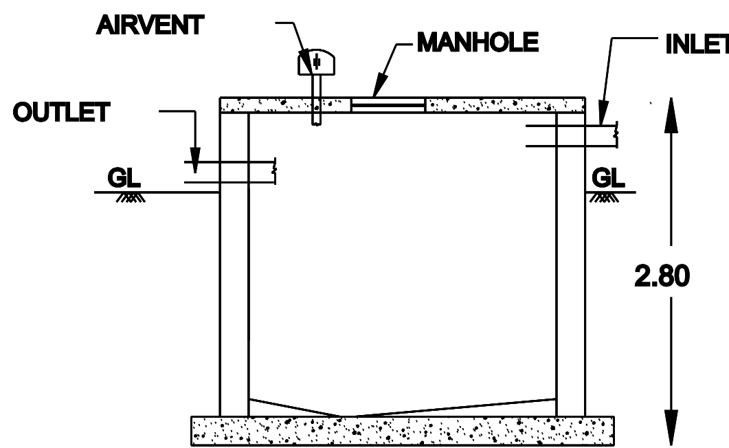
SECTION B-B'
