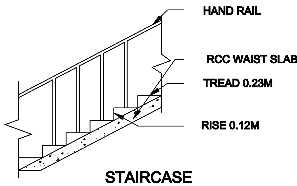
STAIRCASE
