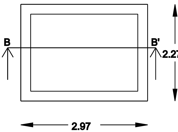
SEPTIC TANK
