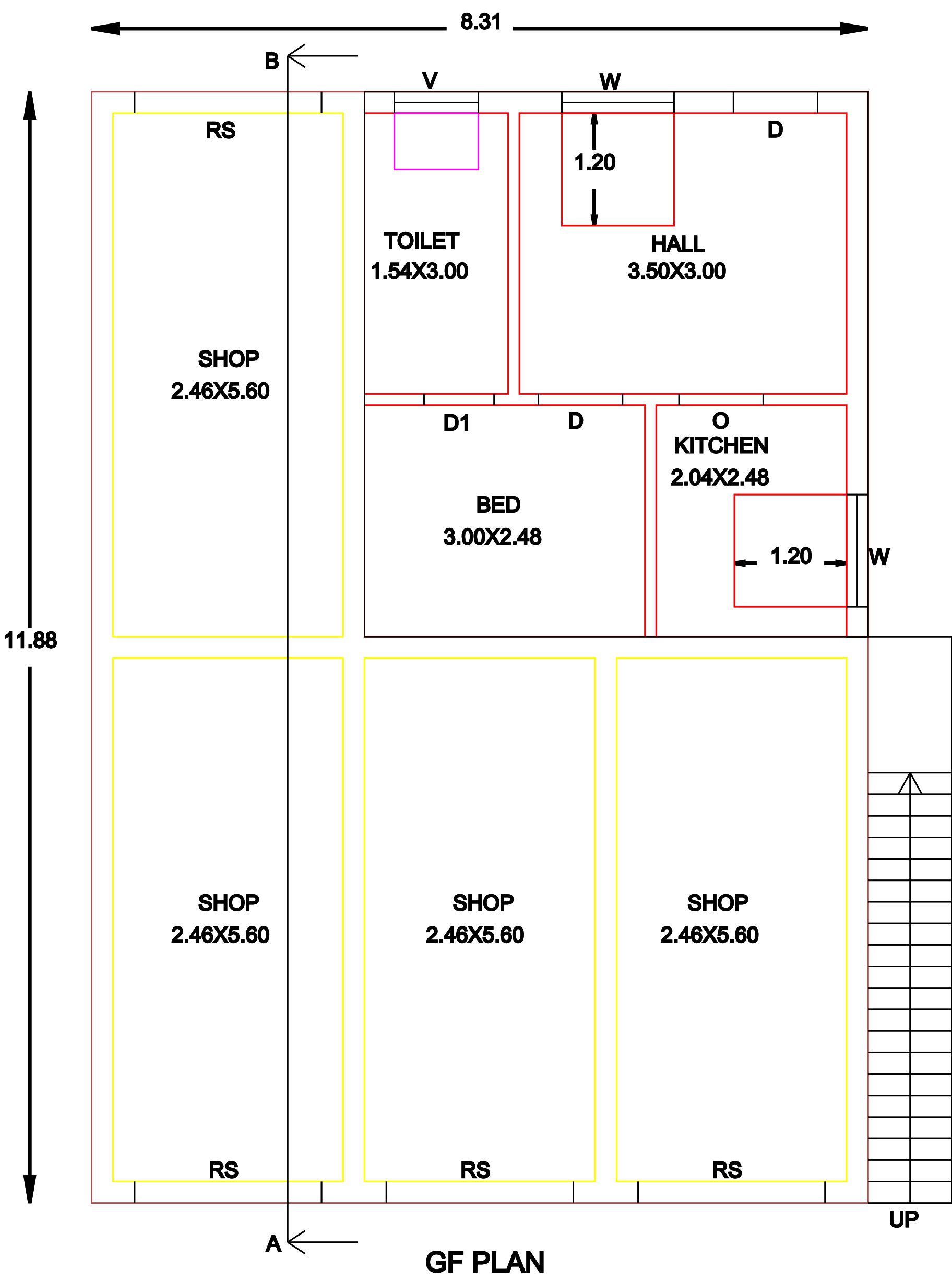
GF PLAN
