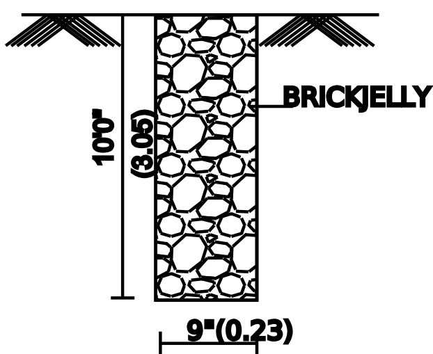
PERCULATION PIT:-
