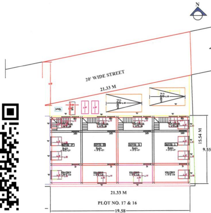
SITE PLAN & G.F. PLAN
