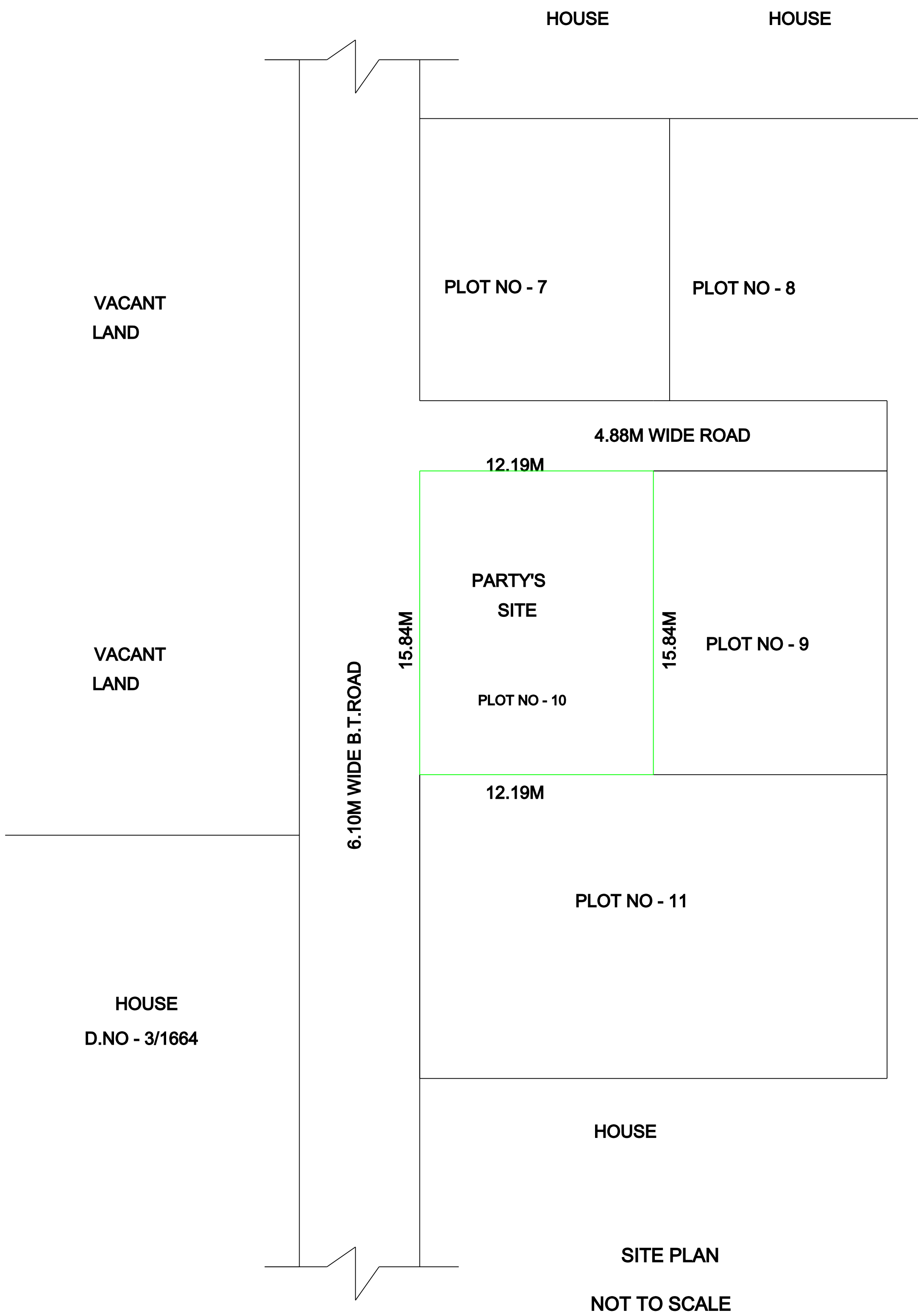
SITE PLAN NOT TO SCALE
