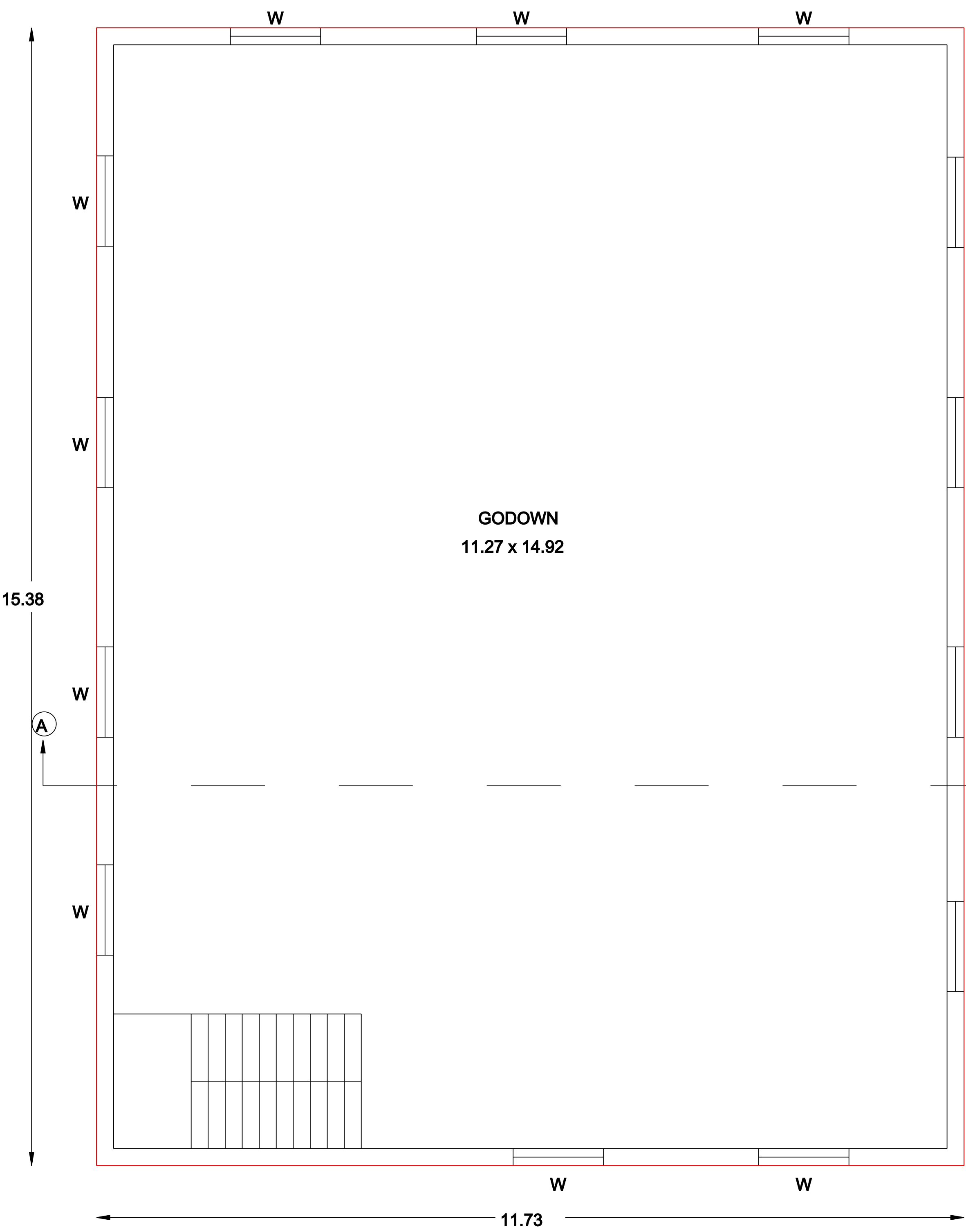
PROPOSED ADDITIOINAL SECOND FLOOR PLAN
