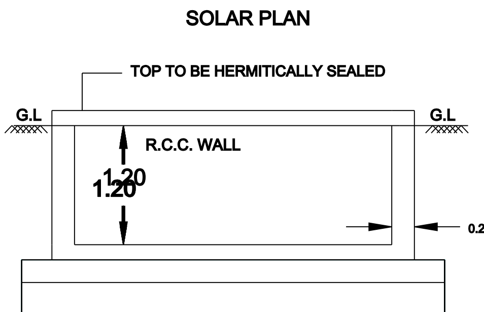
SOLAR PLAN RW H_SECTION
