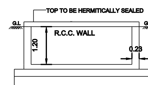
RWY SECTION ( SAMPLE
