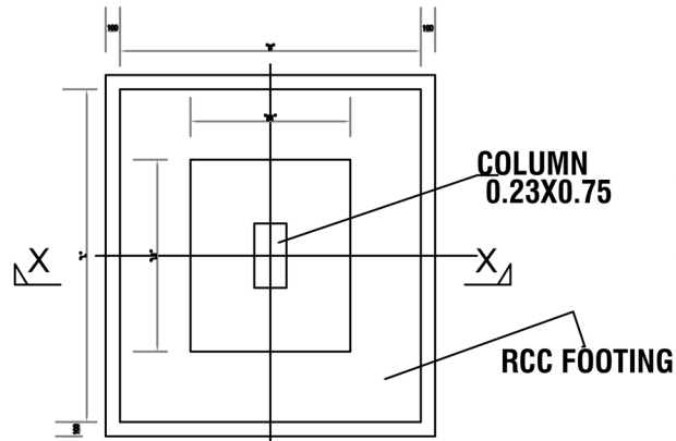
TYP. PLAN OF FOOTING SCALE - 1:75
