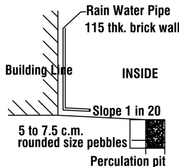
PERCOLATION PIT
