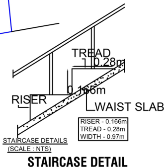
STAIRCASE DETAIL
