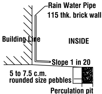
PERCOLATION PIT
