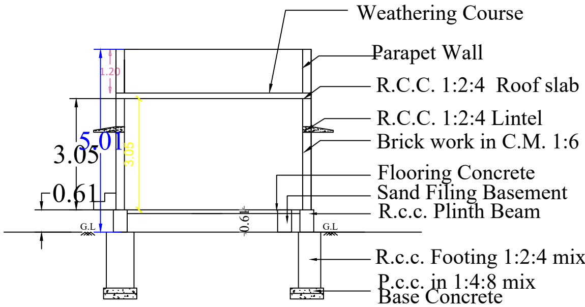
SECTION -"AB"
