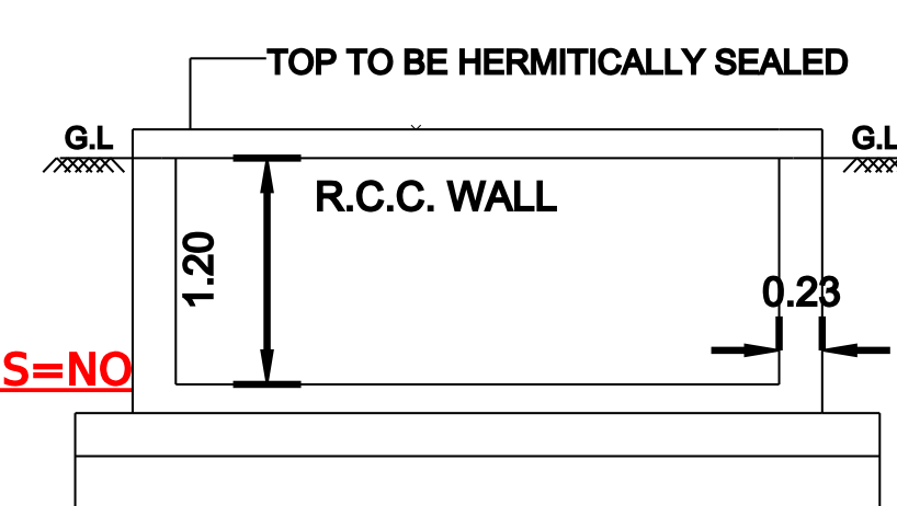
RWI SECTION ( SAMPLE )
