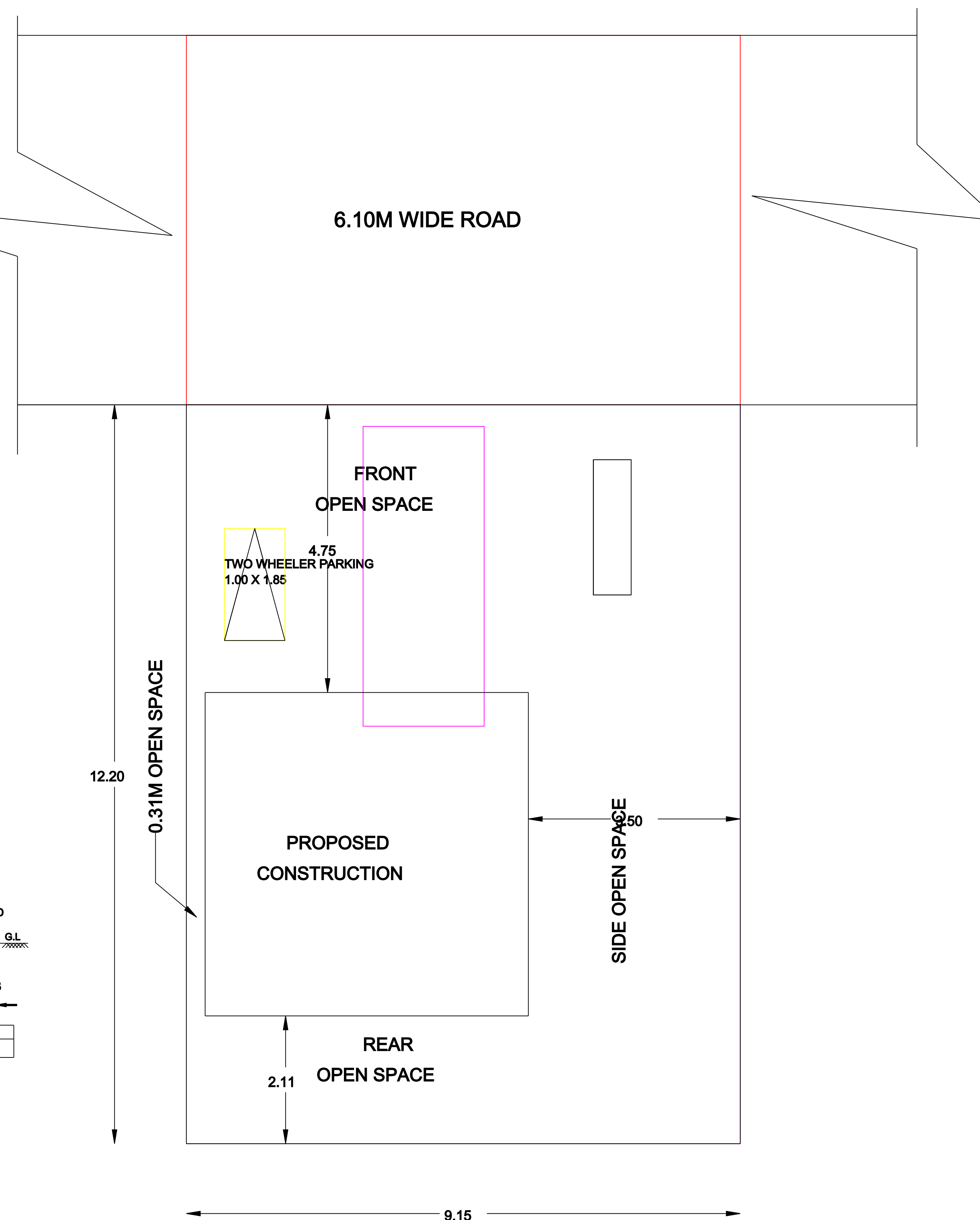
SITE PLAN SCALE :1CM-4M
