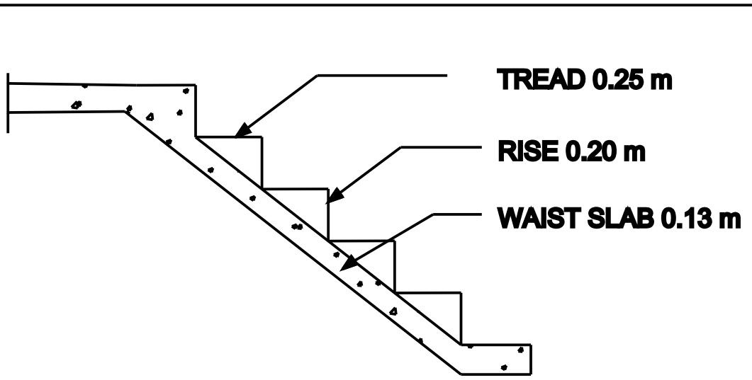
STAIR DETAILS
