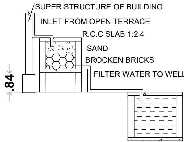
RAINWATER HARVESTING
