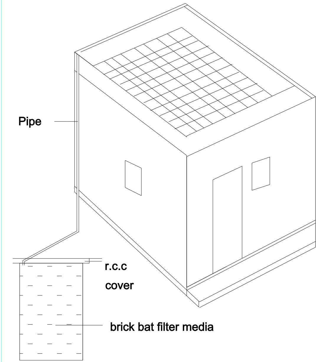
RAIN WATER STORAGE
