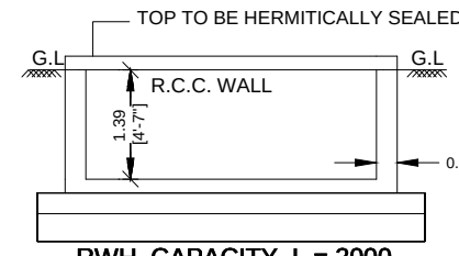
RWH_CAPACITY_L = 2000 RWH SECTION
