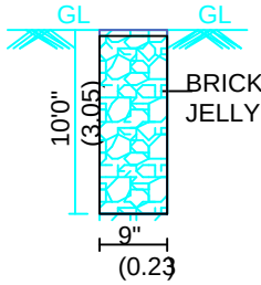
PERCULATION PIT
