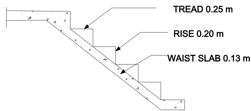
STAIR DETAILS
