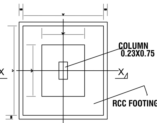
TYP. PLAN OF FOOTING SCALE - 1:75
