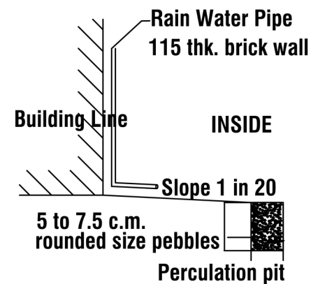
PERCOLATION PIT
