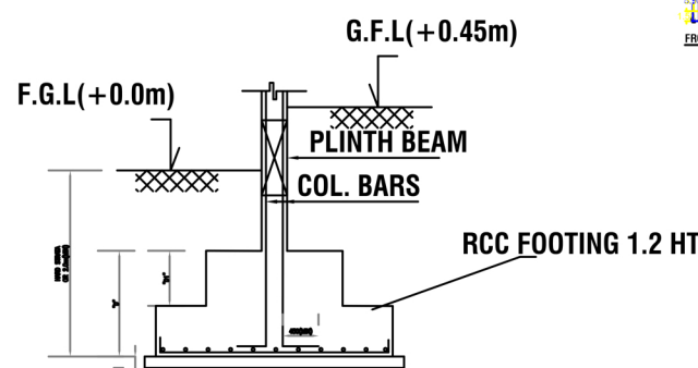
SECTION X-X OF FOOTING SCALE - 1:75
