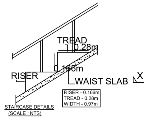
STAIRCASE DETAIL
