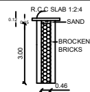
PERCOLATION PIT
