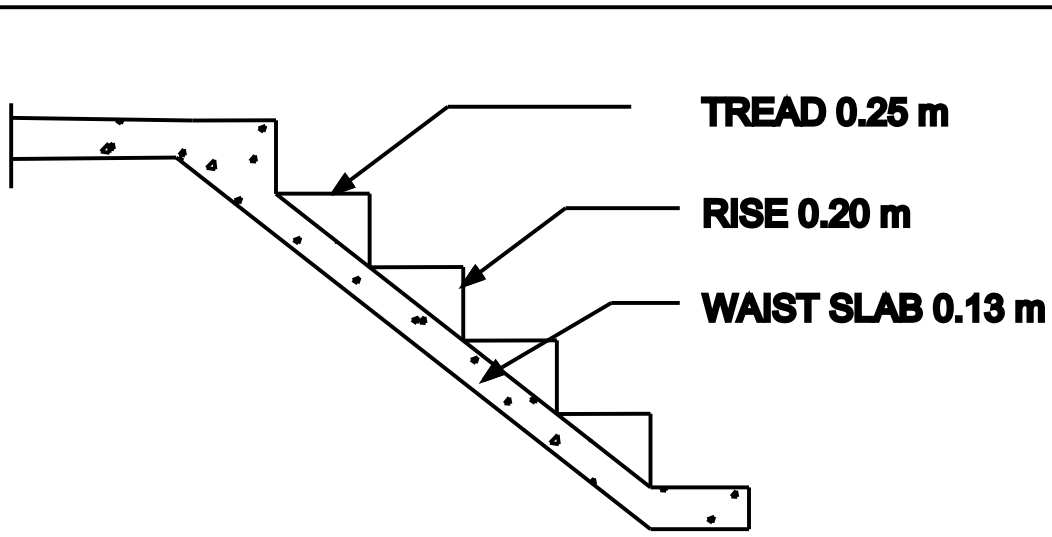
STAIR DETAILS
