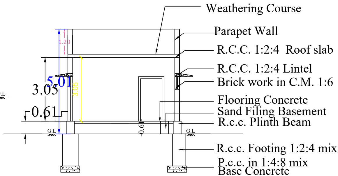
SECTION -"AB"
