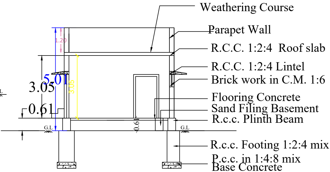
SECTION -"AB"
