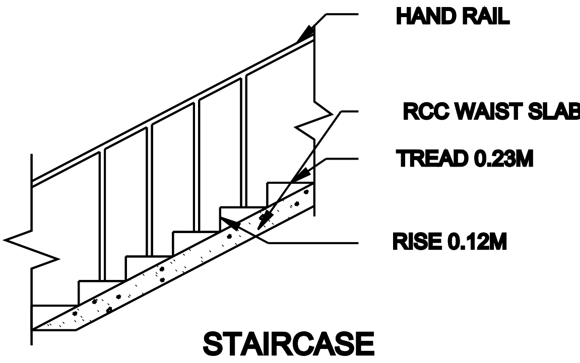
STAIRCASE
