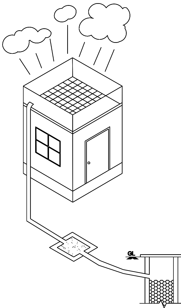
RAINWATER SAVINGS ARRANGEMENTS
