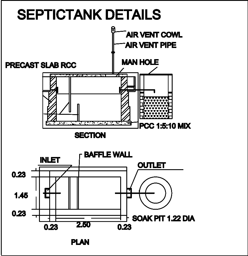
SEPTICTANK DETAILS
