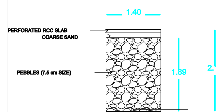
RAIN WATER HARVESTING
