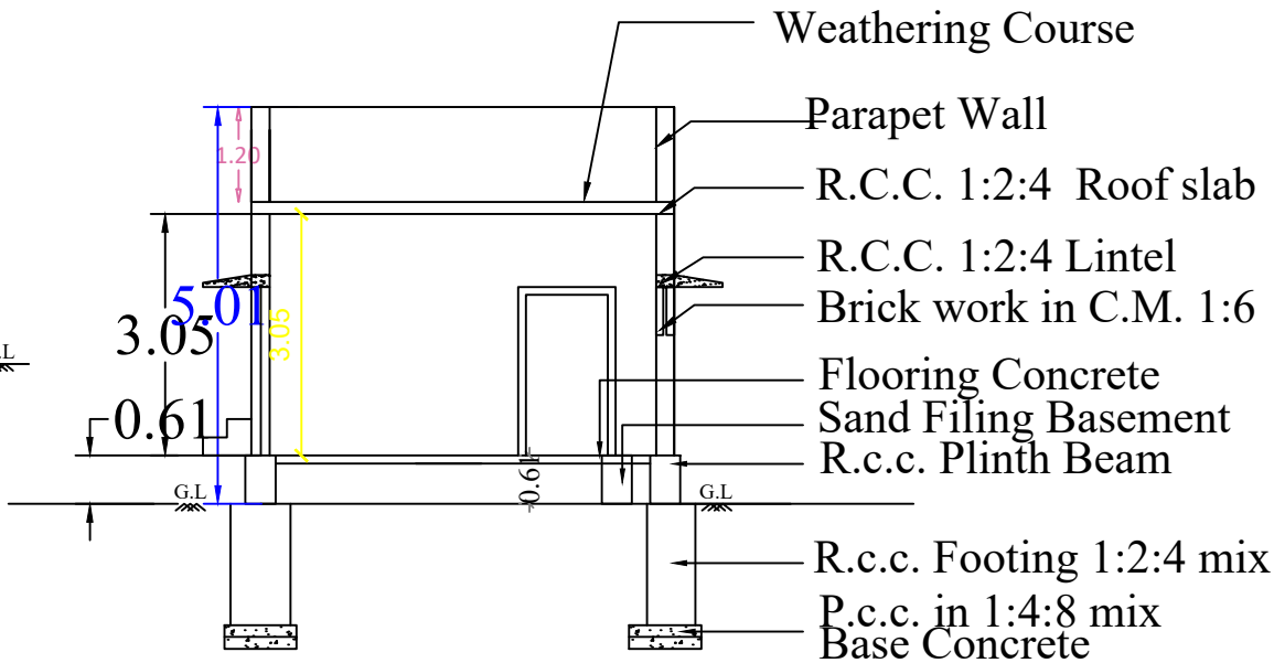
SECTION -"AB"
