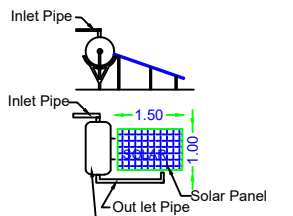
DETAILS OF SOLAR WATER HEATER
