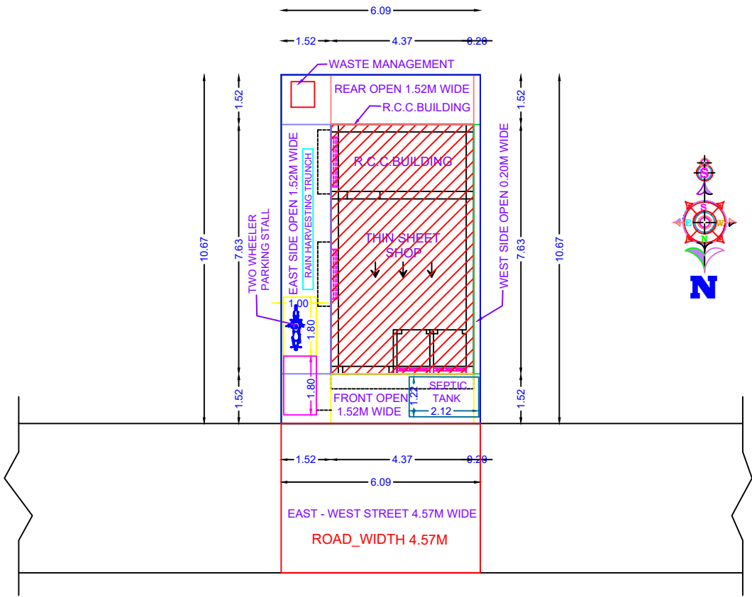
SITE PLAN
