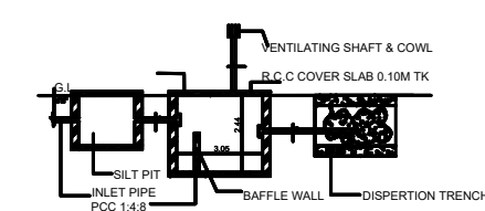
'U' TRAPS SEPTIC TANK DETAILS
