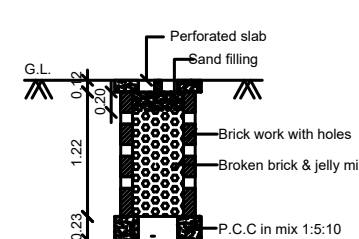
PERCOLATION PIT (Scale:- 1:50)
