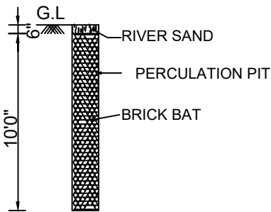
PERCOLATION PIT
