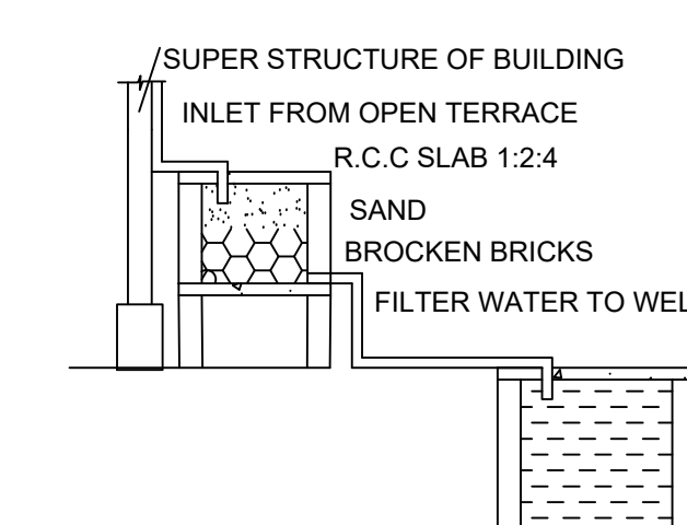
RAINWATER HARVESTING
